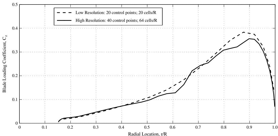
Fig. 9 Comparison of the loading on the main rotor blades when at an azimuth of 90°, computed using two different combinations of blade discretization and grid cell density. The tail rotor is configured in the low position with a top-forward sense of rotation. Advance ratio = 0.07.
