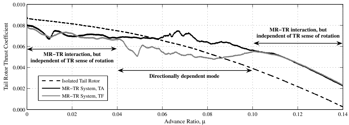
Fig. 3 Variation in the thrust coefficient developed by the low tail rotor as the MR-TR system accelerates gradually along a 60° sideslip trajectory (TA: top-aft tail rotor, TF: top-forward tail rotor).
