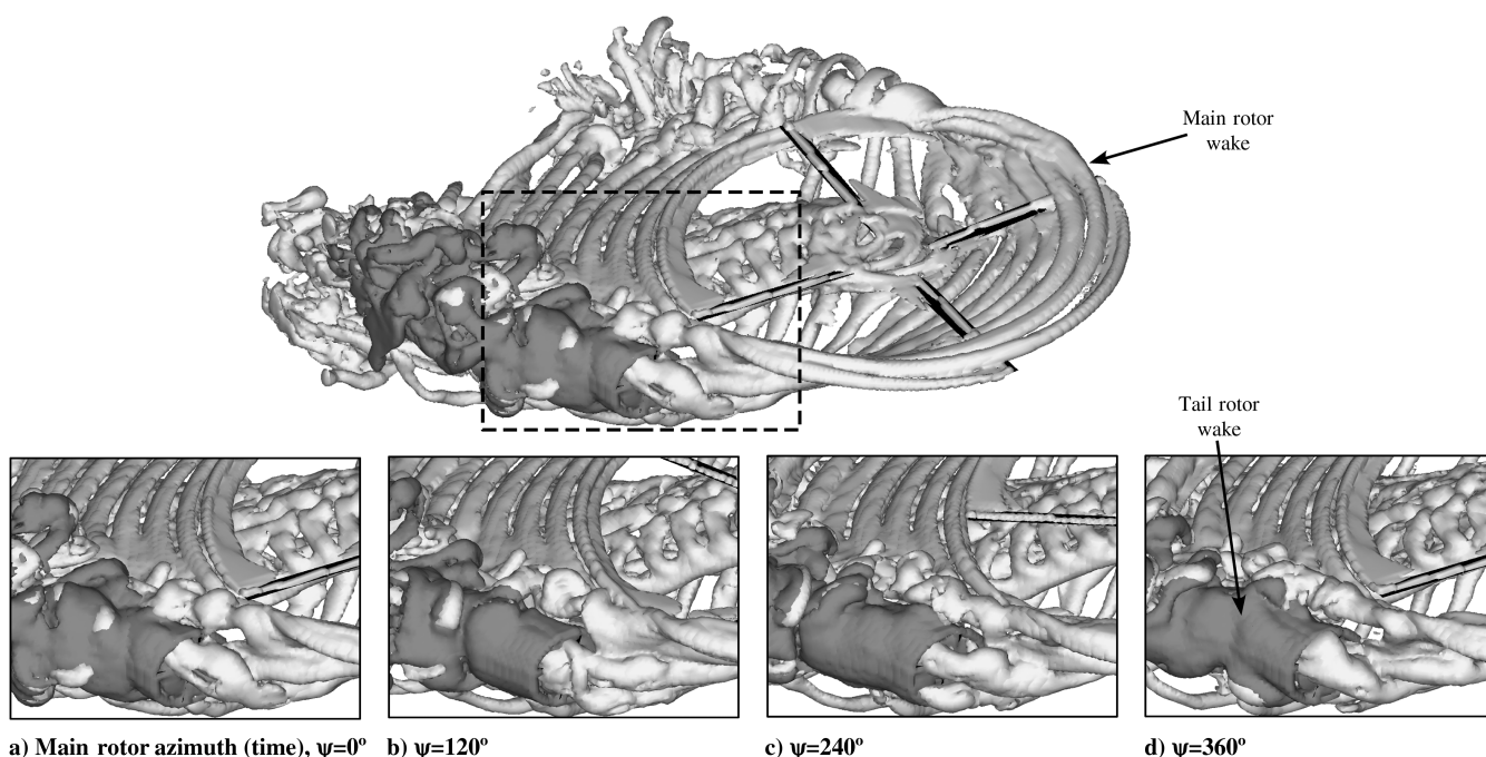
Fig. 10 Highly resolved instantaneous snapshot of the wake of a low tail rotor operating with the main rotor in 60^\circ sideslip at an advance ratio of 0.07 (light surface, main rotor wake; dark surface, tail rotor wake).
